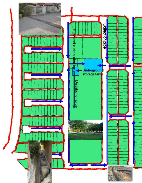
Figure 2. Proposed RWHS within Taman Wangsa Melawati
